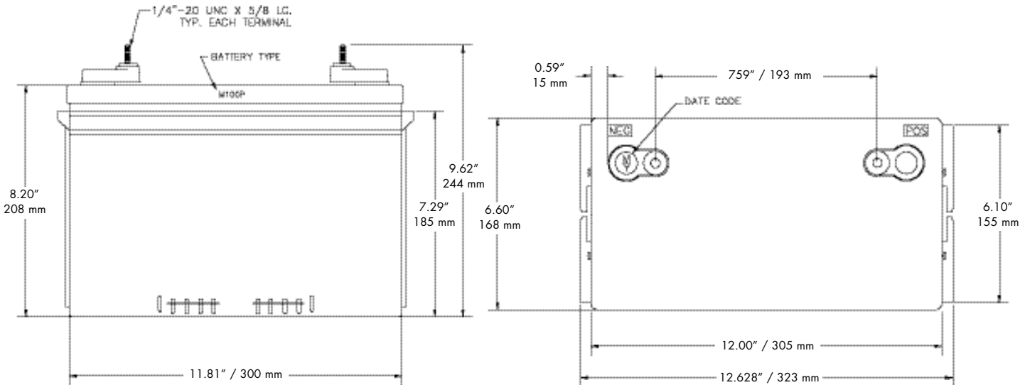
SIDE VIEW
