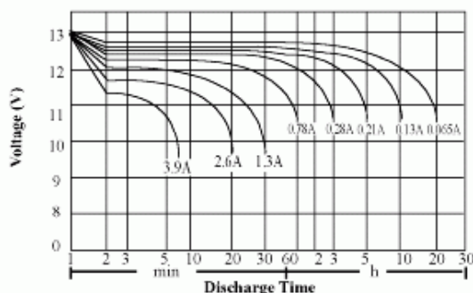
Discharge Characteristics fully charged (25°C/77°F)
