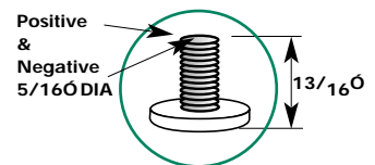
5/16 Studs
